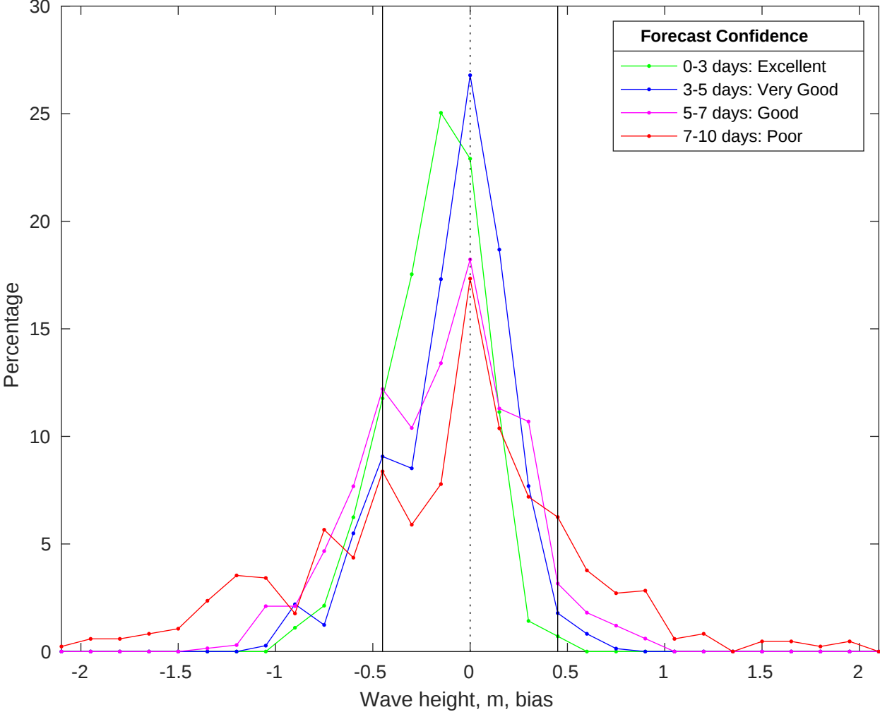
NDBC 46069 vs CMEMS Waves Bias Histogram: 20-Oct-2025
