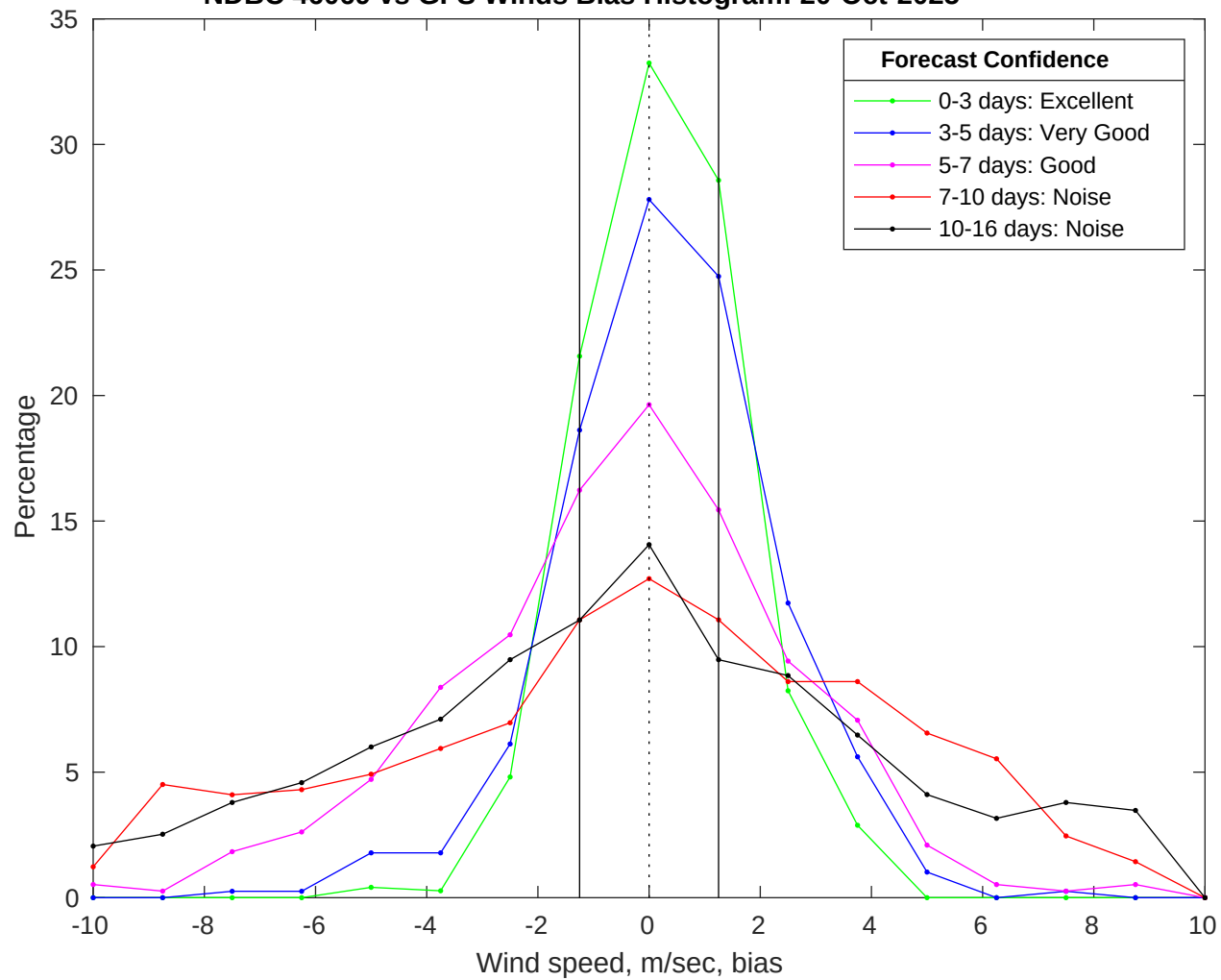
NDBC 46069 vs GFS Winds Bias Histogram: 20-Oct-2025
