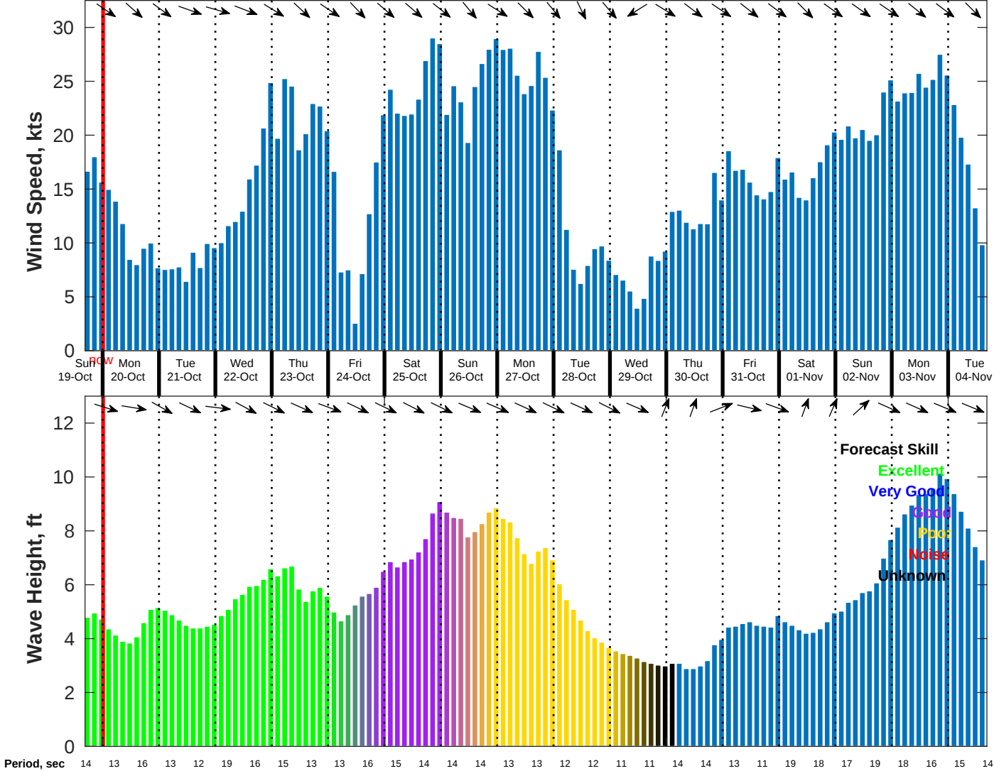
Wind & Wave Forecast for NDBC 46069 from 19-Oct-2025 16:00:00 to 04-Nov-2025 16:00:00
