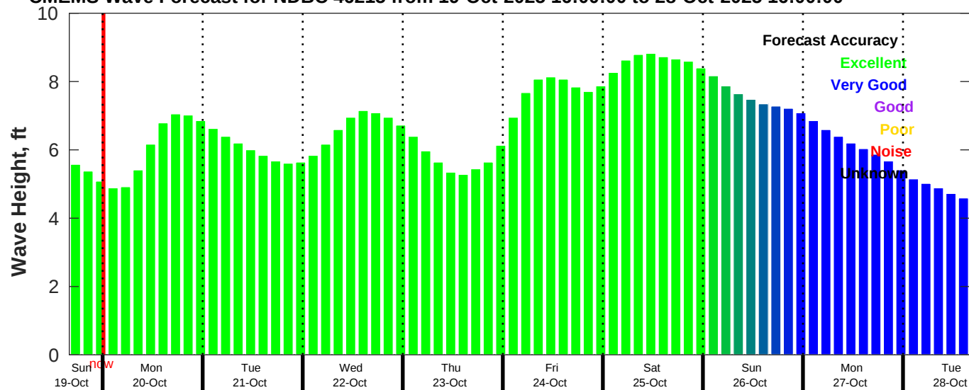
CMEMS Wave Forecast for NDBC 46215 from 19-Oct-2025 16:00:00 to 28-Oct-2025 16:00:00
