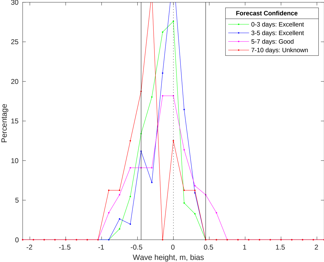
NDBC 46259 vs CMEMS Waves Bias Histogram: 20-Oct-2025
