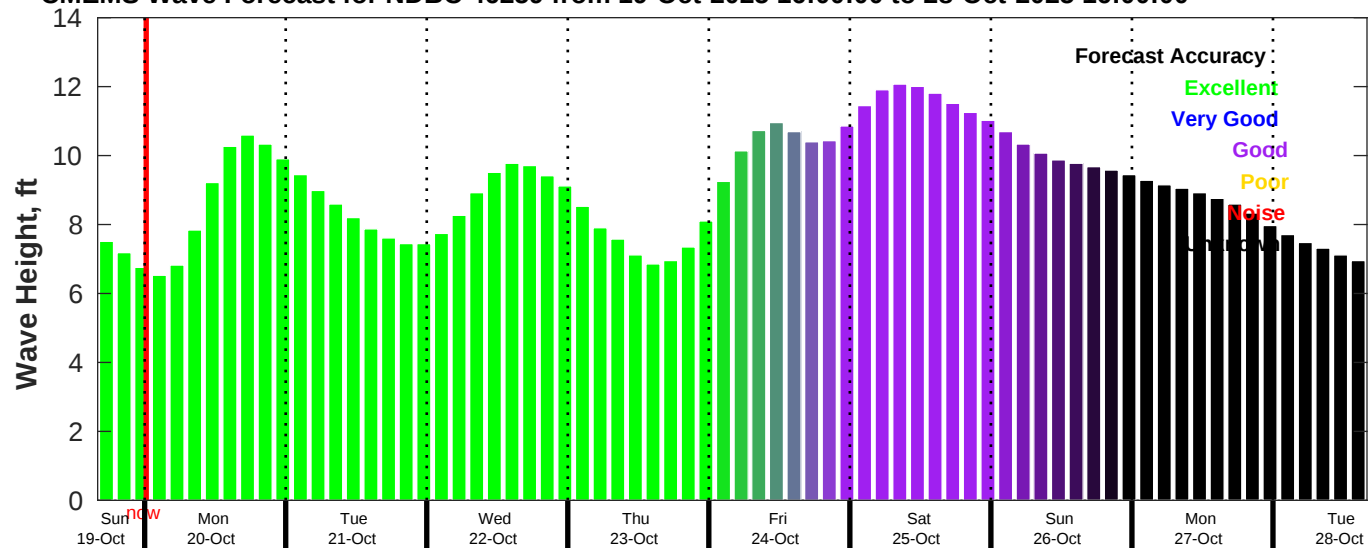
CMEMS Wave Forecast for NDBC 46259 from 19-Oct-2025 16:00:00 to 28-Oct-2025 16:00:00
