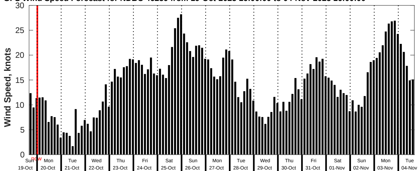
GFS Wind Speed Forecast for NDBC 46259 from 19-Oct-2025 16:00:00 to 04-Nov-2025 16:00:00
