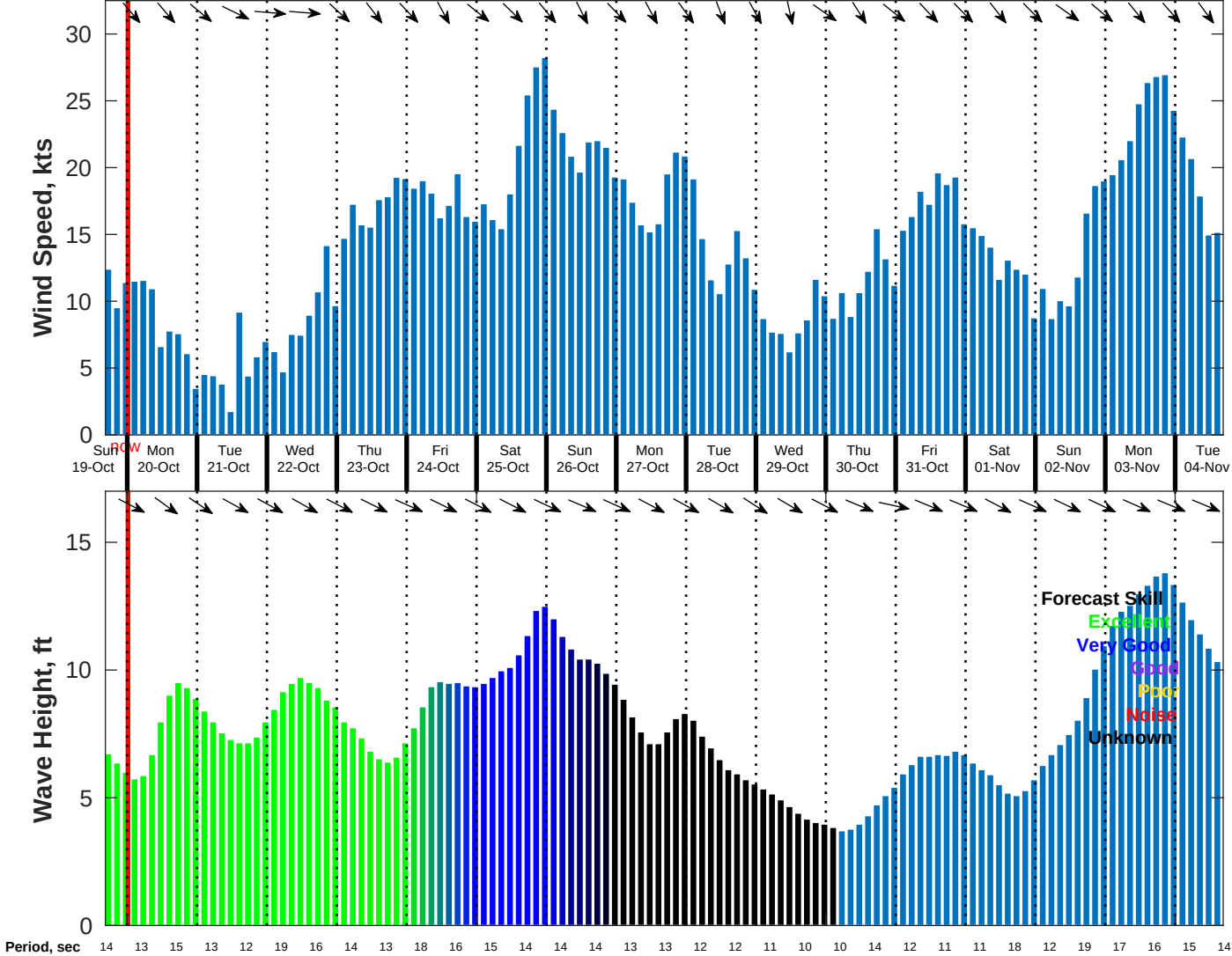
Wind & Wave Forecast for NDBC 46259 from 19-Oct-2025 16:00:00 to 04-Nov-2025 16:00:00
