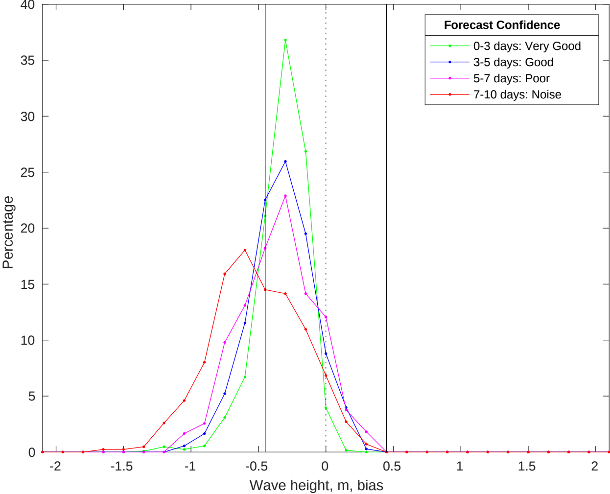
NDBC 51209 vs CMEMS Waves Bias Histogram: 20-Oct-2025
