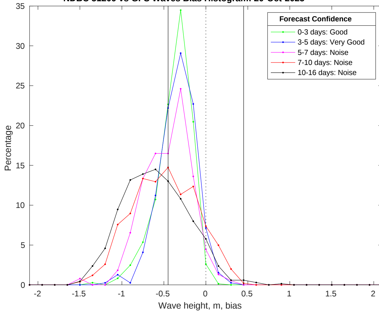
NDBC 51209 vs GFS Waves Bias Histogram: 20-Oct-2025
