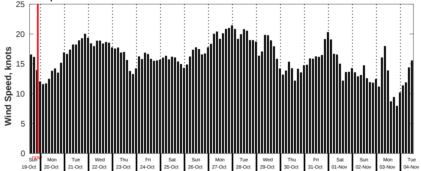
GFS Wind Speed Forecast for NDBC 51209 from 19-Oct-2025 13:00:00 to 04-Nov-2025 13:00:00
