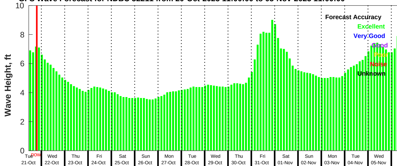
GFS Wave Forecast for NDBC 52211 from 20-Oct-2025 11:00:00 to 05-Nov-2025 11:00:00
