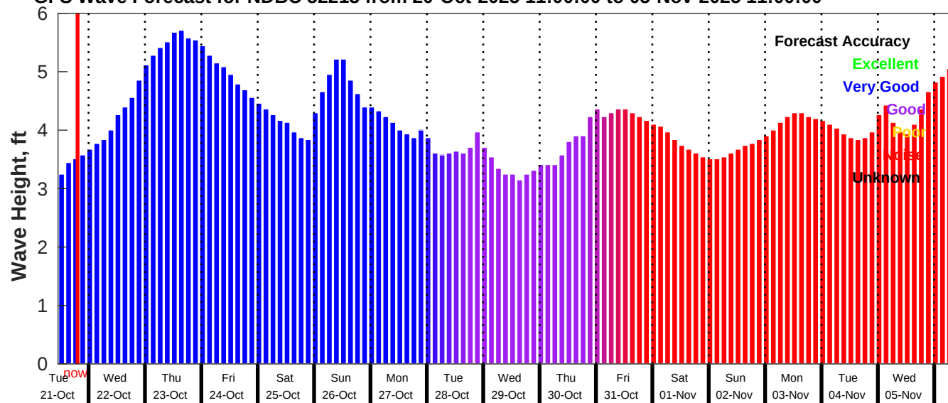
GFS Wave Forecast for NDBC 52213 from 20-Oct-2025 11:00:00 to 05-Nov-2025 11:00:00
