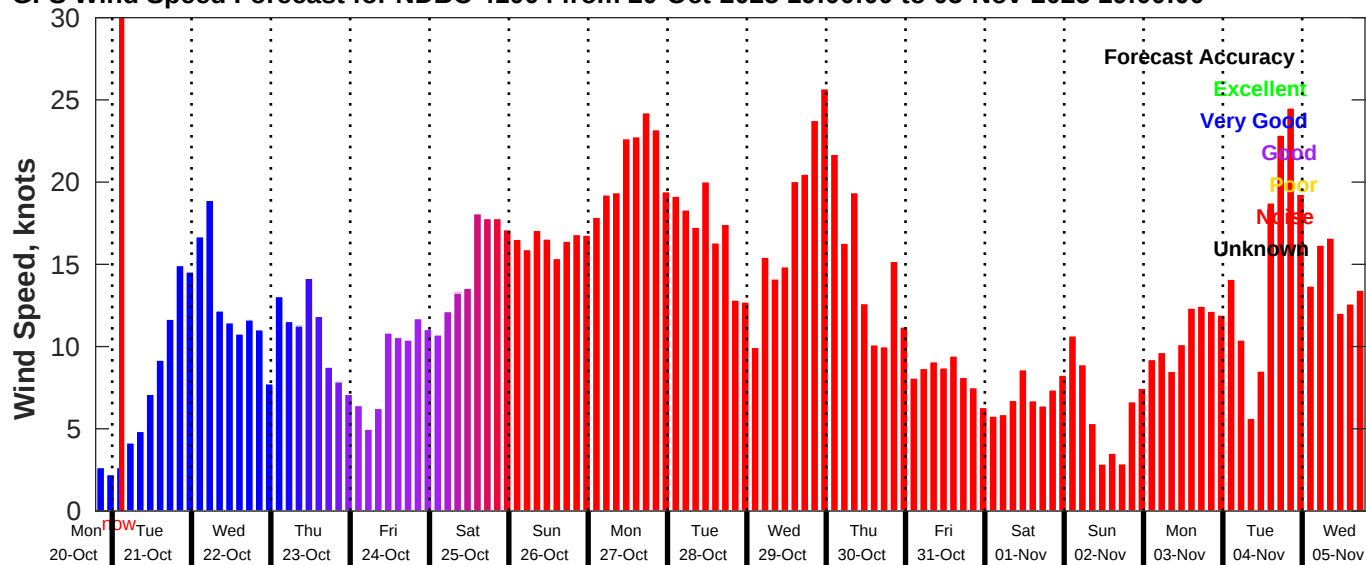
GFS Wind Speed Forecast for NDBC 41004 from 20-Oct-2025 19:00:00 to 05-Nov-2025 19:00:00
