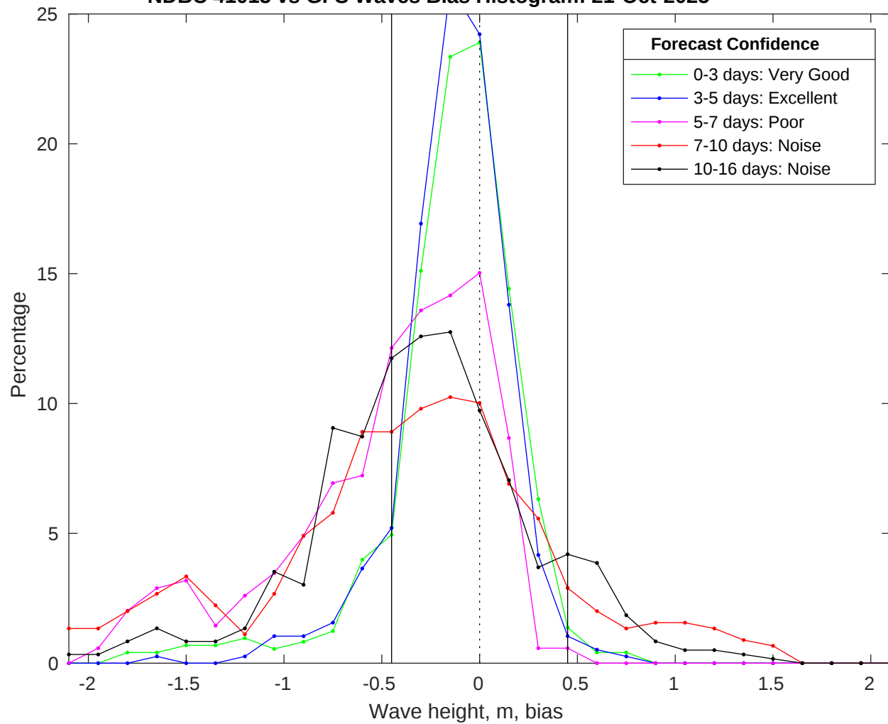
NDBC 41013 vs GFS Waves Bias Histogram: 21-Oct-2025
