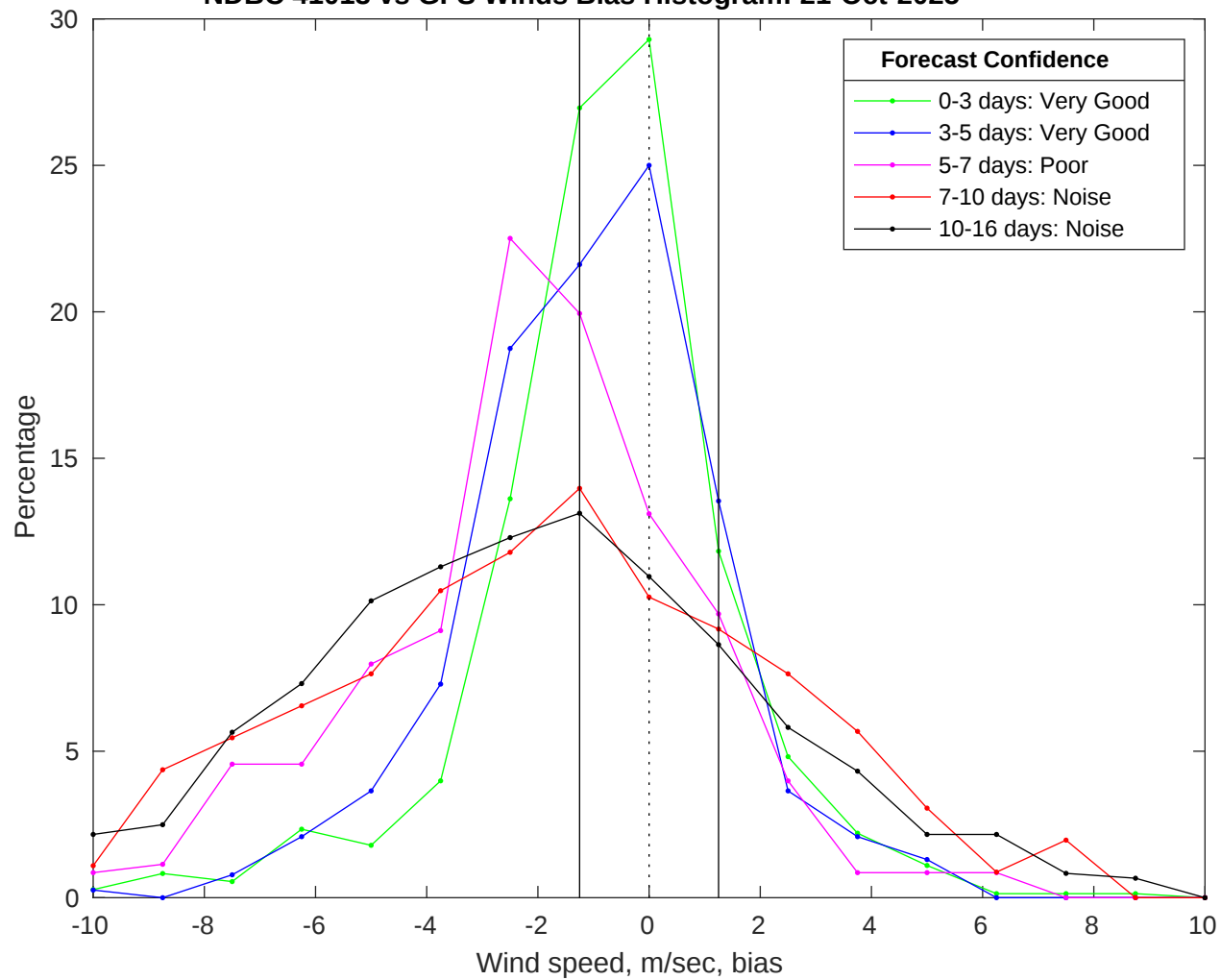
NDBC 41013 vs GFS Winds Bias Histogram: 21-Oct-2025
