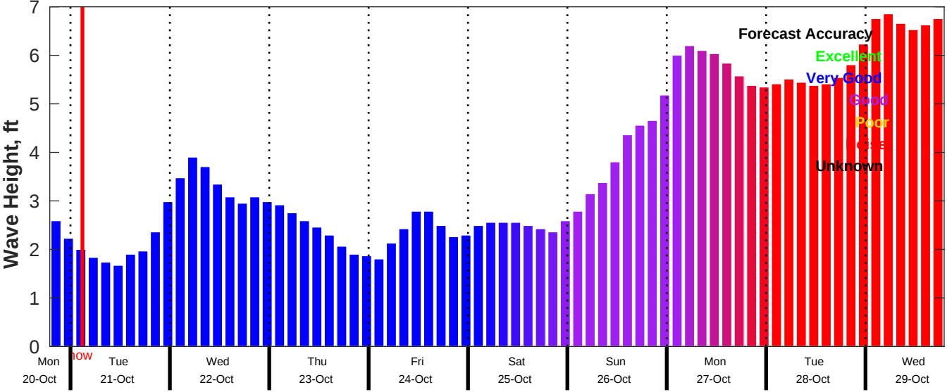
CMEMS Wave Forecast for NDBC 41013 from 20-Oct-2025 19:00:00 to 29-Oct-2025 19:00:00
