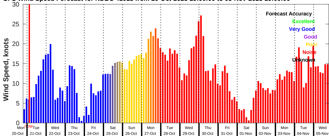
GFS Wind Speed Forecast for NDBC 41013 from 20-Oct-2025 19:00:00 to 05-Nov-2025 19:00:00
