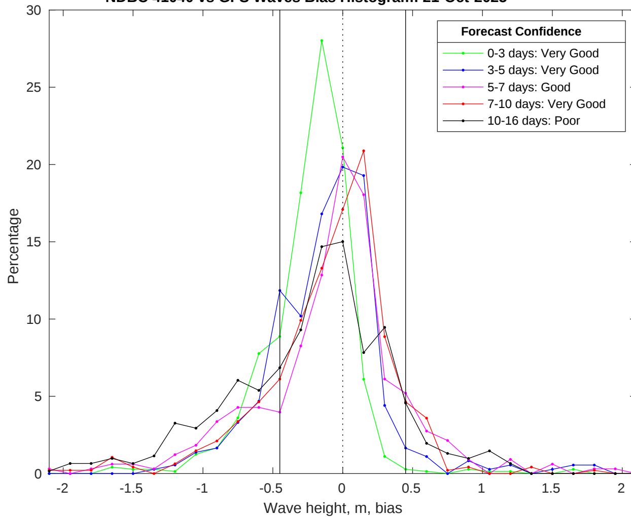
NDBC 41040 vs GFS Waves Bias Histogram: 21-Oct-2025
