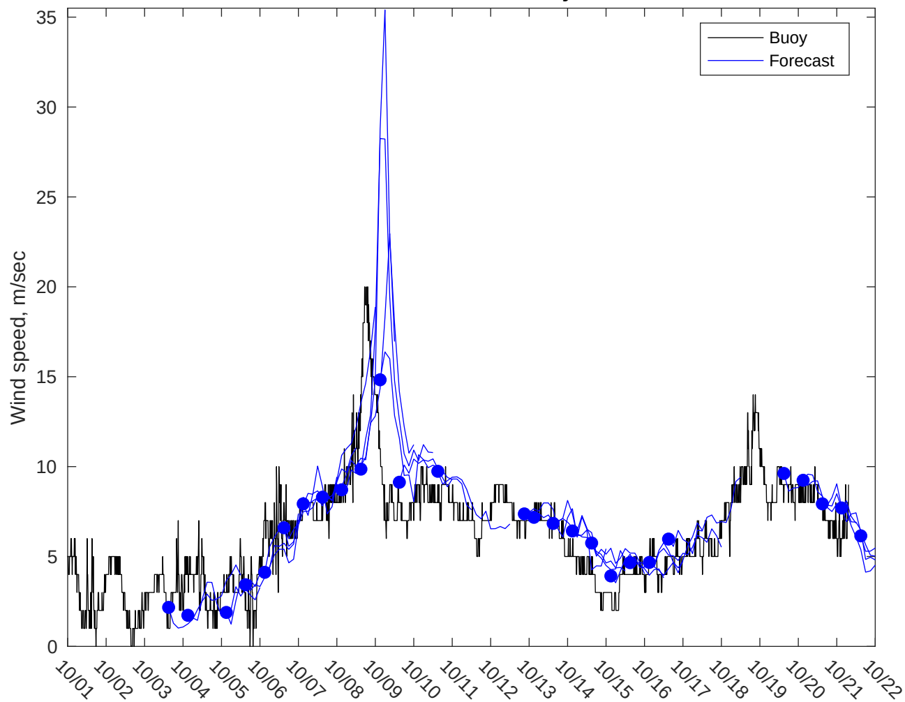
NDBC 41040 vs GFS Winds: 3 to 5 day forecast
