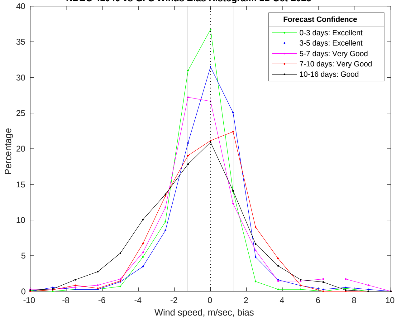
NDBC 41040 vs GFS Winds Bias Histogram: 21-Oct-2025
