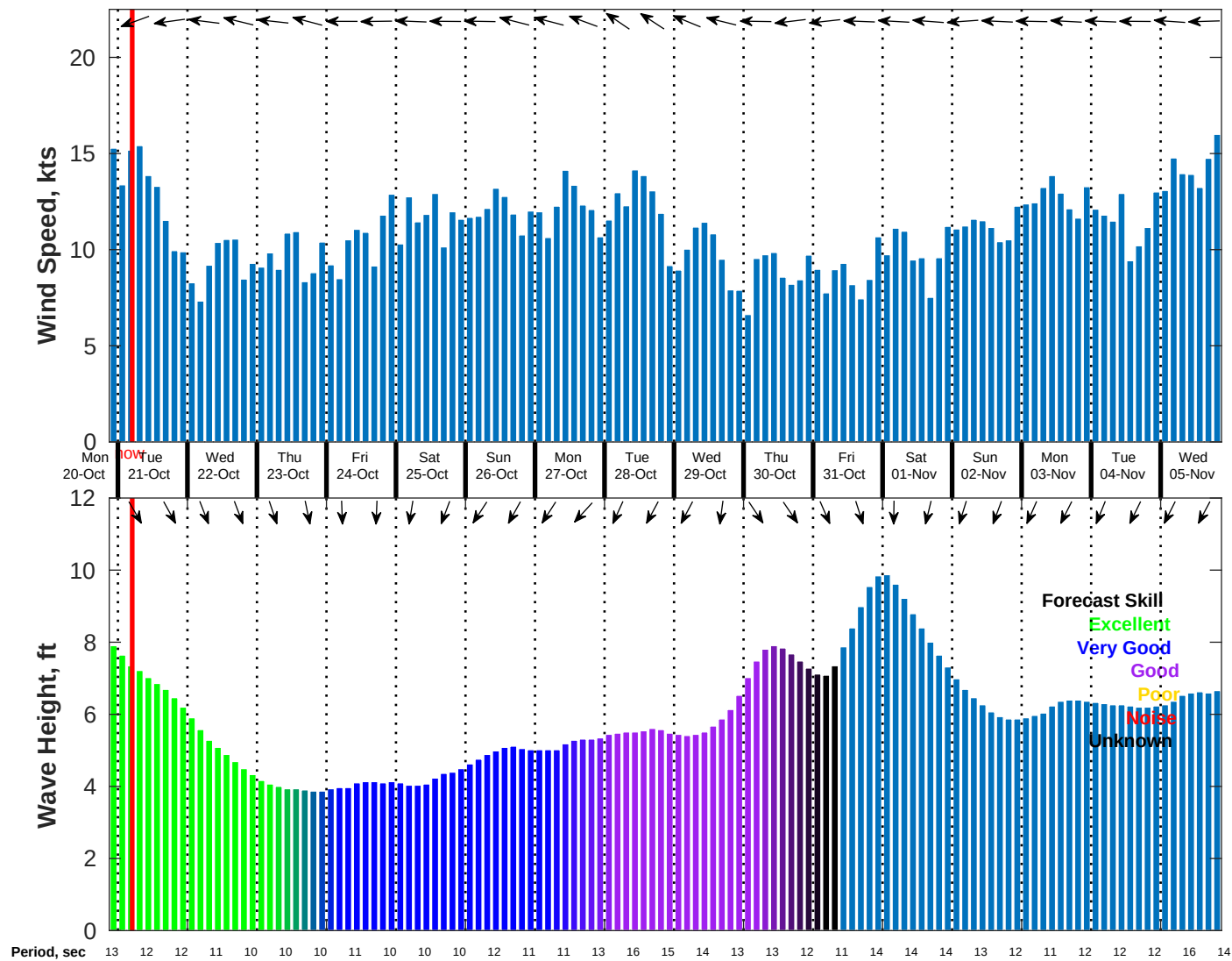
Wind & Wave Forecast for NDBC 41040 from 20-Oct-2025 21:00:00 to 05-Nov-2025 21:00:00
