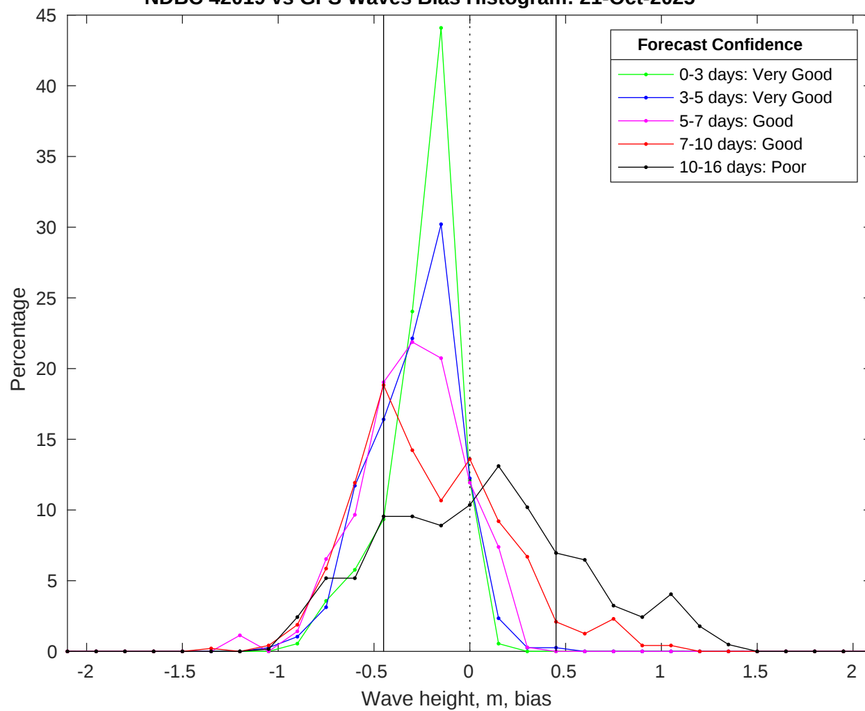
NDBC 42019 vs GFS Waves Bias Histogram: 21-Oct-2025
