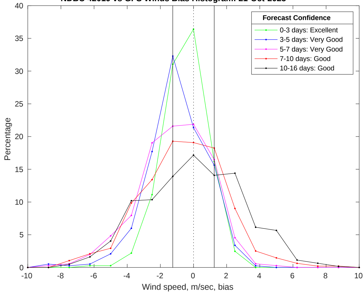
NDBC 42019 vs GFS Winds Bias Histogram: 21-Oct-2025
