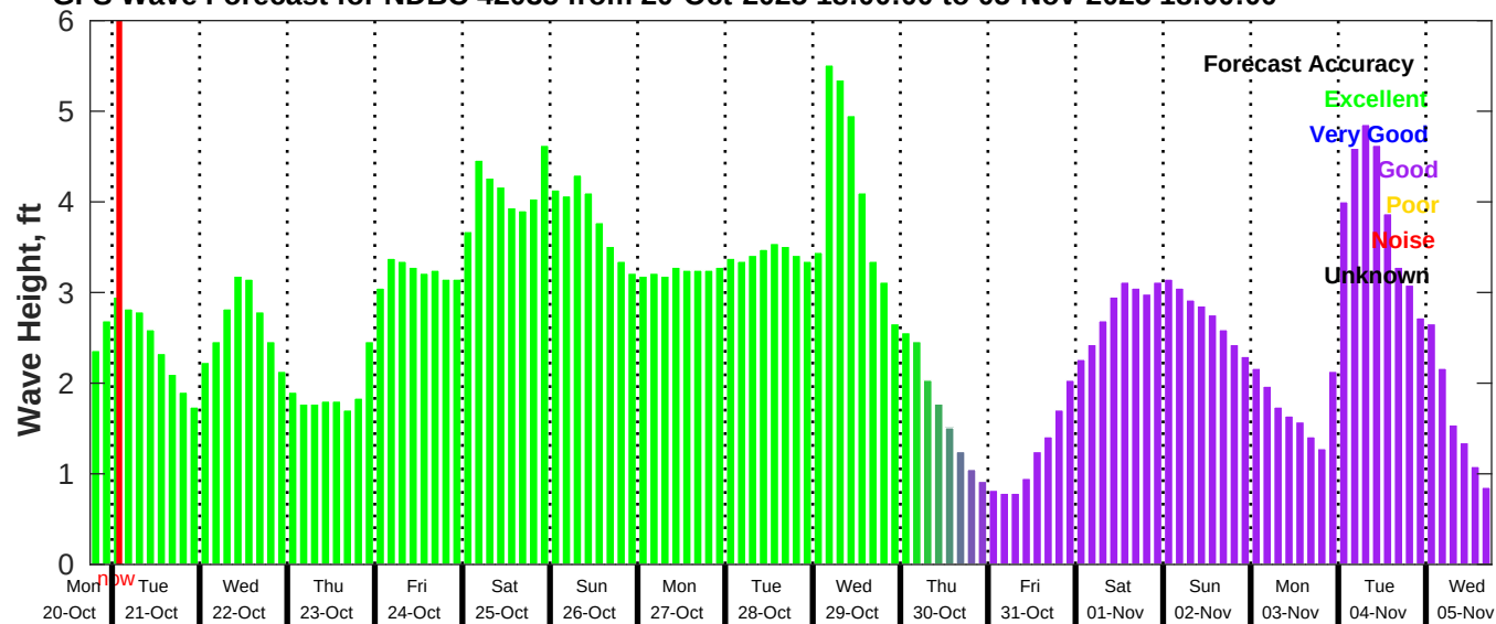
GFS Wave Forecast for NDBC 42035 from 20-Oct-2025 18:00:00 to 05-Nov-2025 18:00:00
