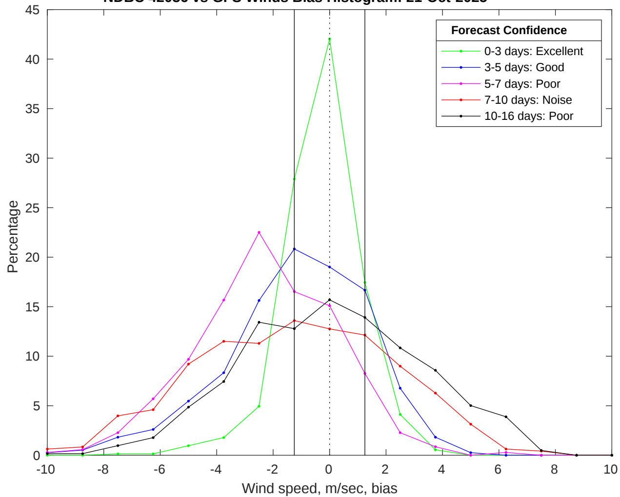
NDBC 42036 vs GFS Winds Bias Histogram: 21-Oct-2025
