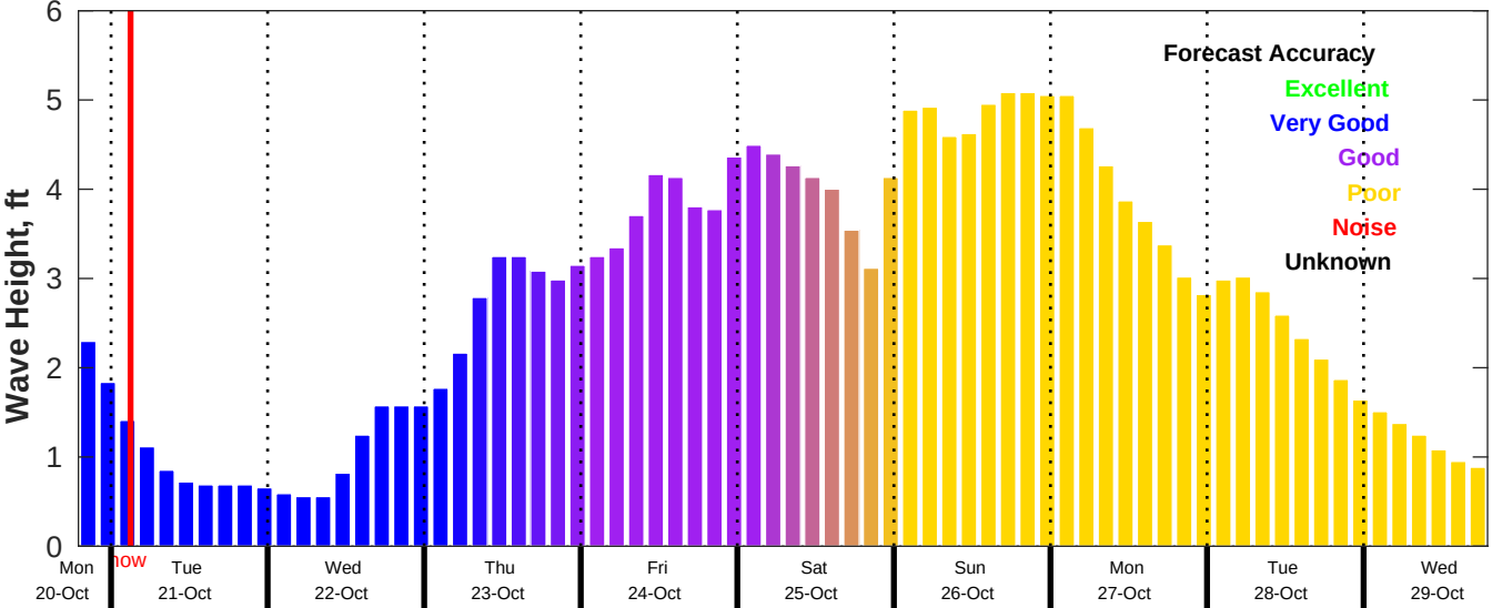
CMEMS Wave Forecast for NDBC 42036 from 20-Oct-2025 19:00:00 to 29-Oct-2025 19:00:00
