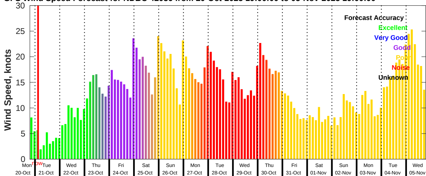
GFS Wind Speed Forecast for NDBC 42036 from 20-Oct-2025 19:00:00 to 05-Nov-2025 19:00:00
