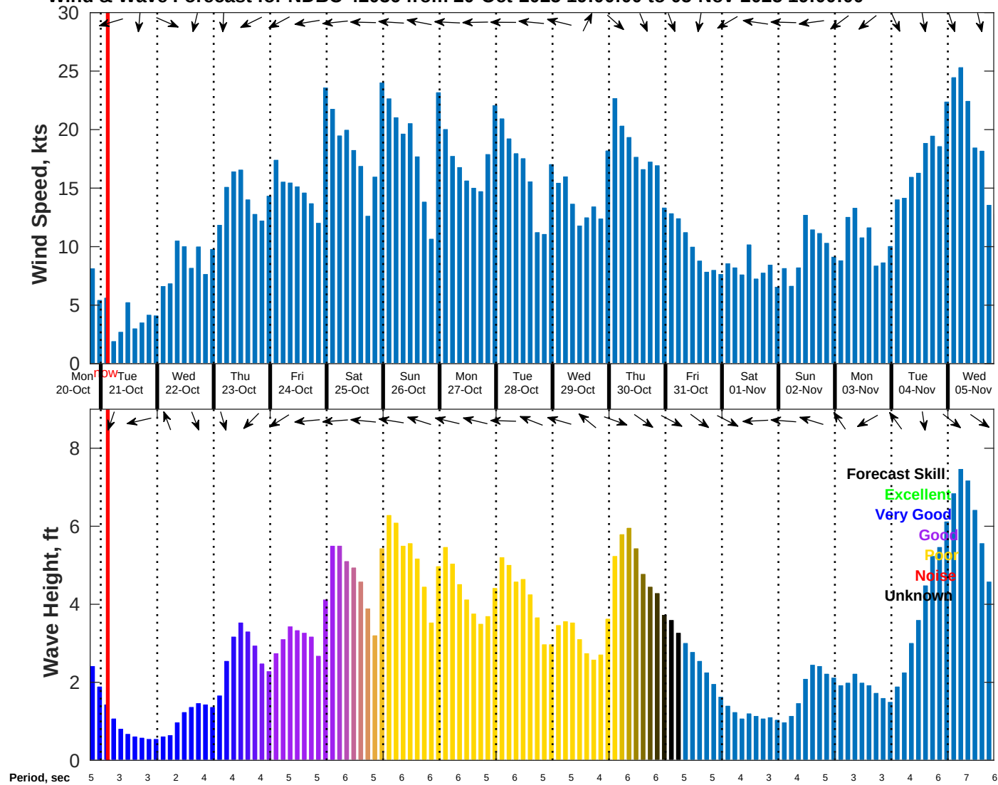
Wind & Wave Forecast for NDBC 42036 from 20-Oct-2025 19:00:00 to 05-Nov-2025 19:00:00
