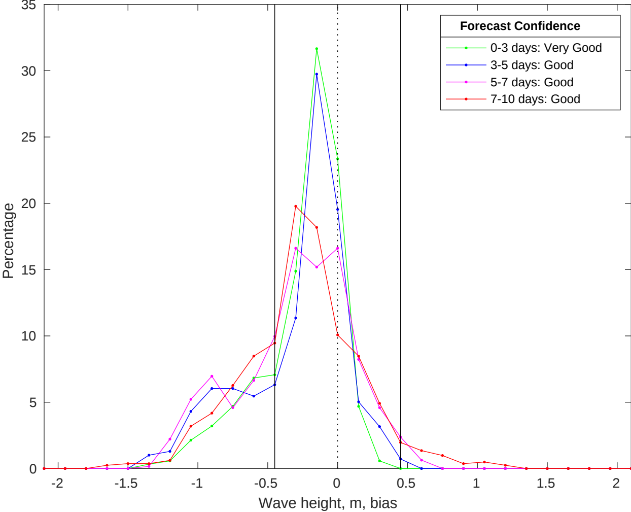
NDBC 42040 vs CMEMS Waves Bias Histogram: 21-Oct-2025
