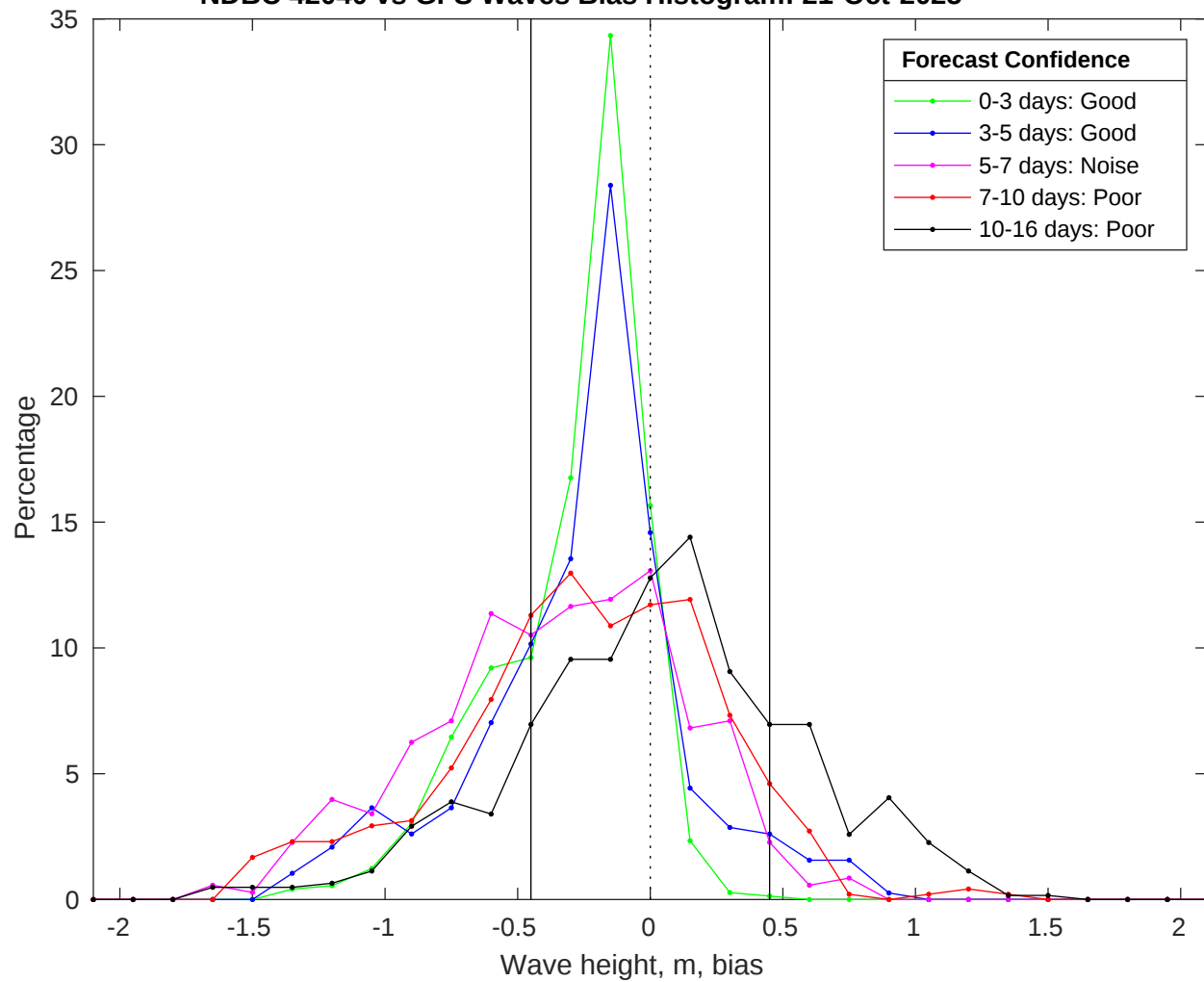
NDBC 42040 vs GFS Waves Bias Histogram: 21-Oct-2025
