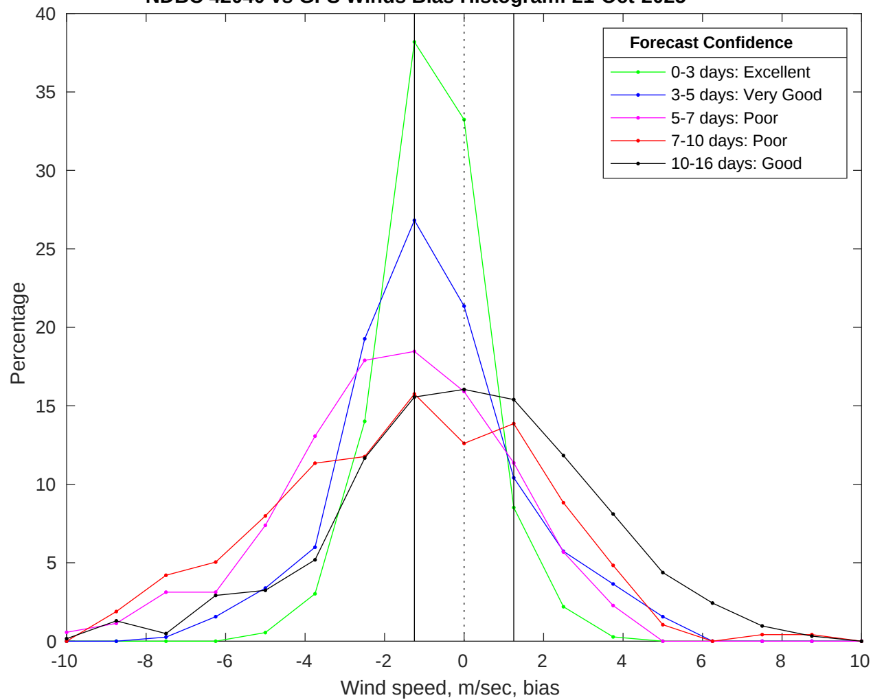
NDBC 42040 vs GFS Winds Bias Histogram: 21-Oct-2025
