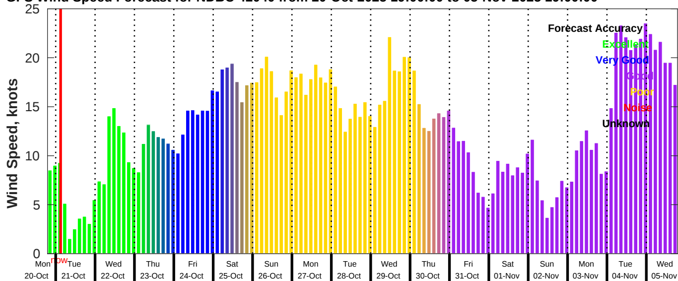
GFS Wind Speed Forecast for NDBC 42040 from 20-Oct-2025 19:00:00 to 05-Nov-2025 19:00:00
