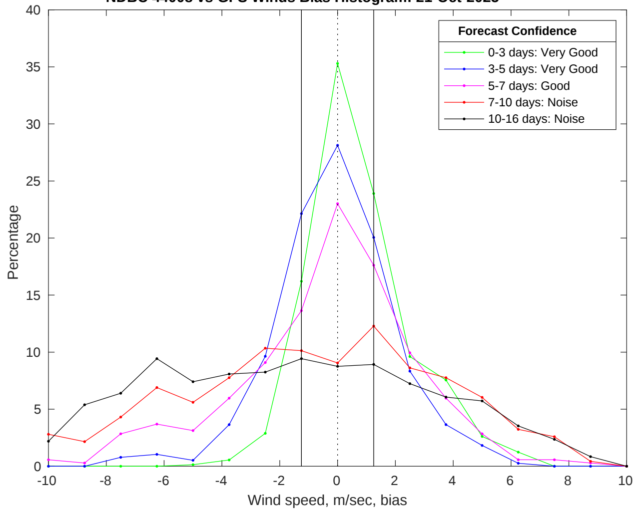
NDBC 44008 vs GFS Winds Bias Histogram: 21-Oct-2025
