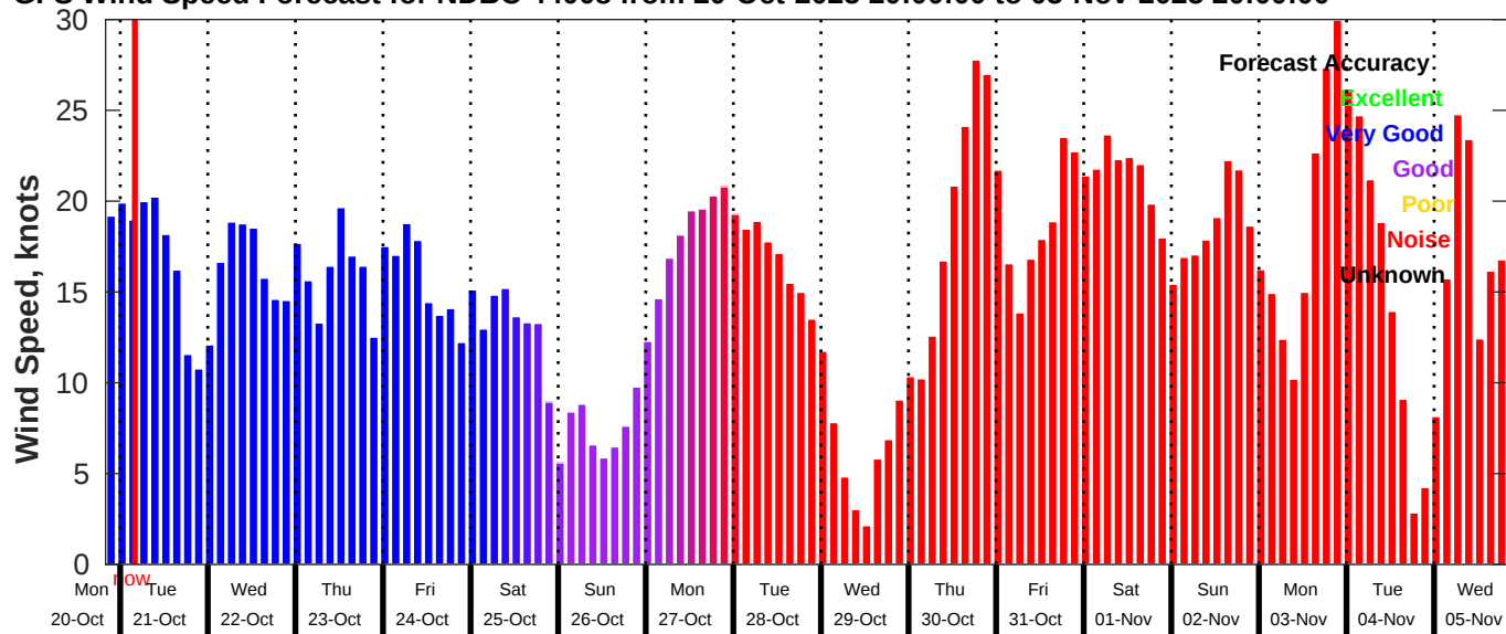
GFS Wind Speed Forecast for NDBC 44008 from 20-Oct-2025 20:00:00 to 05-Nov-2025 20:00:00
