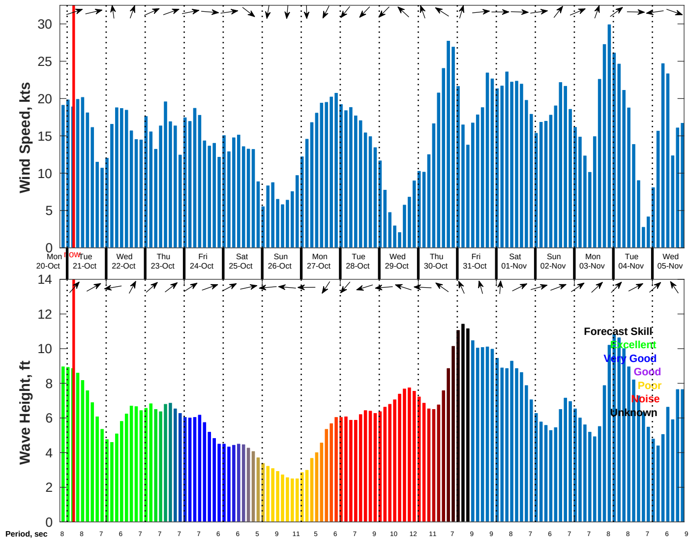
Wind & Wave Forecast for NDBC 44008 from 20-Oct-2025 20:00:00 to 05-Nov-2025 20:00:00
