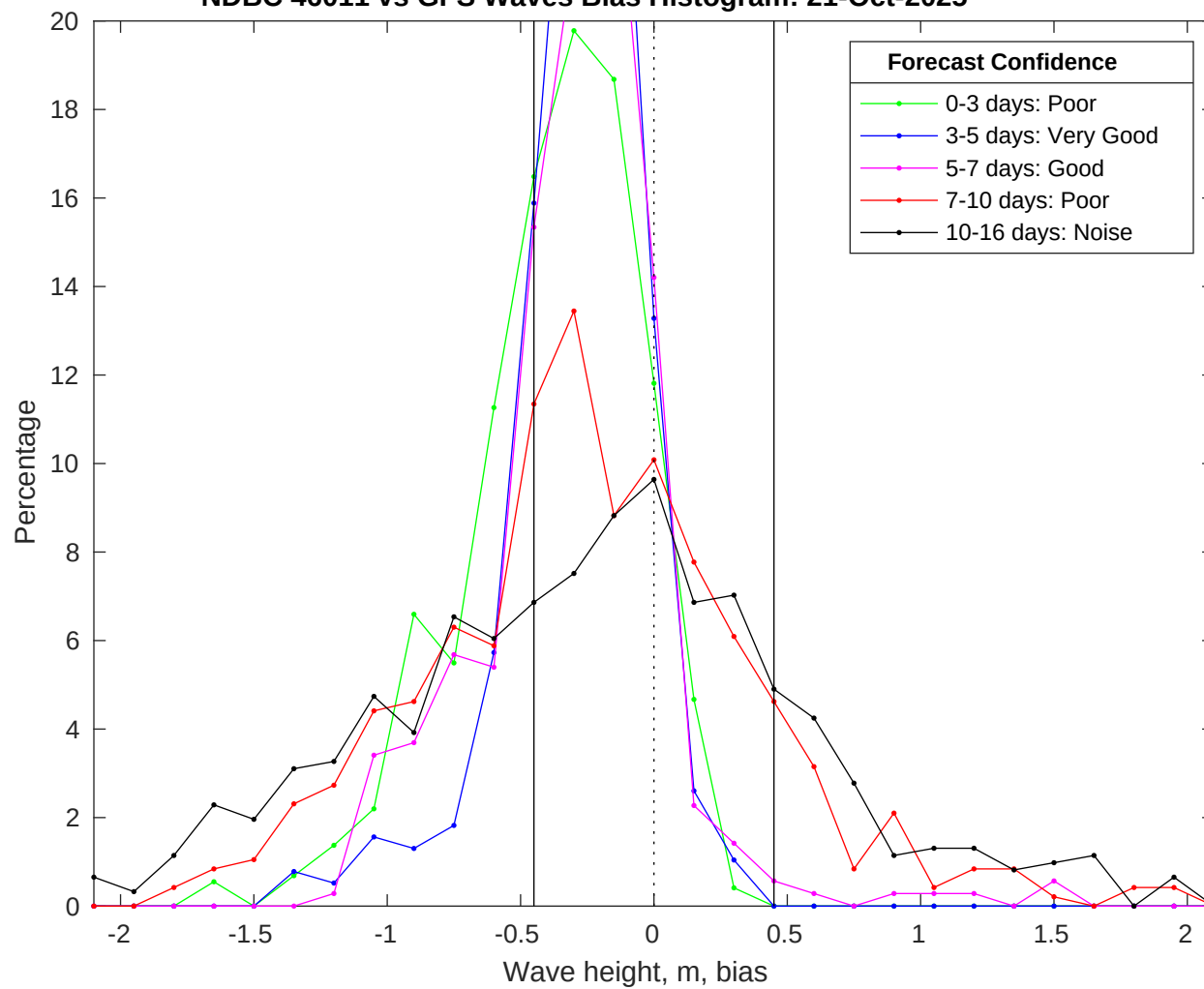
NDBC 46011 vs GFS Waves Bias Histogram: 21-Oct-2025
