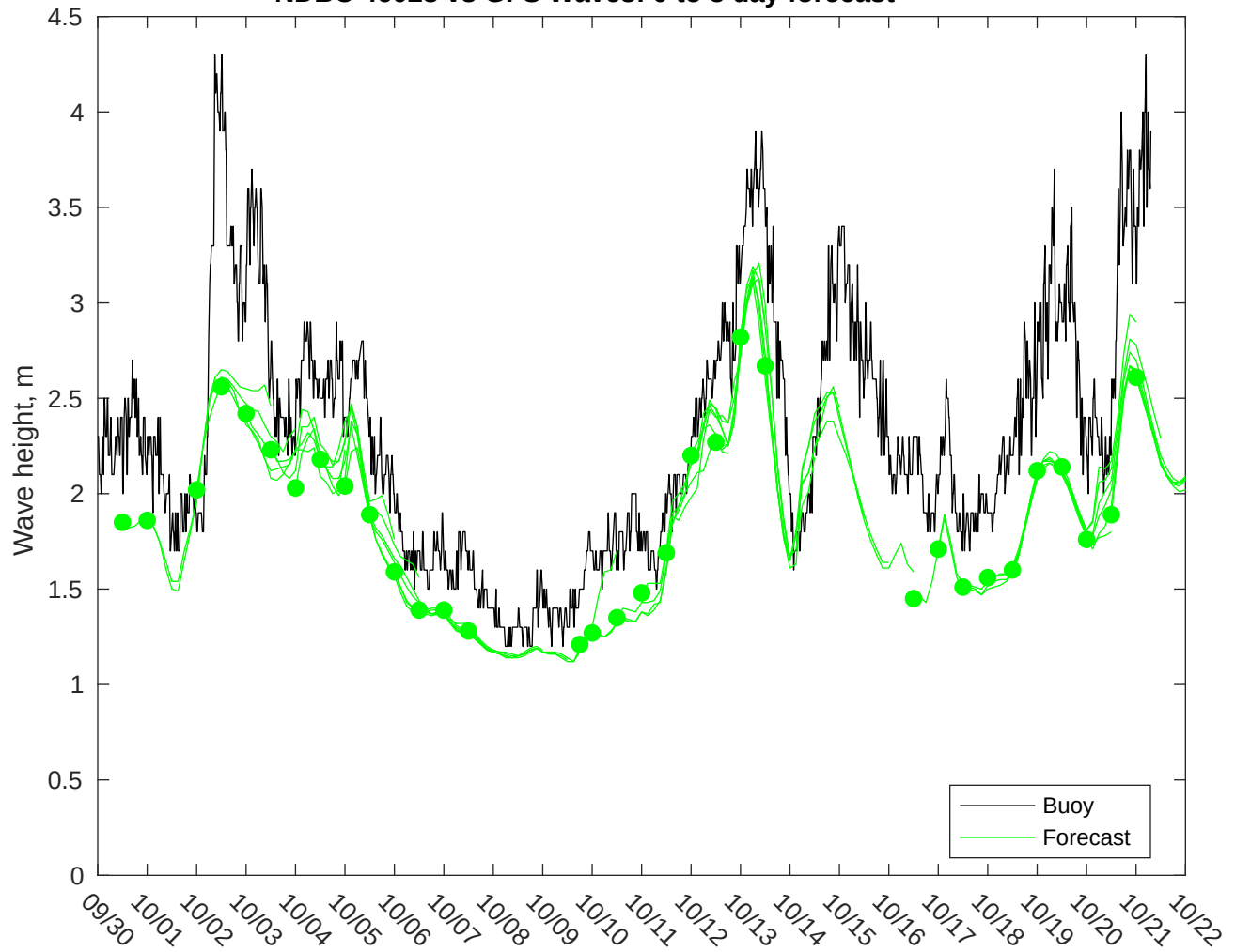
NDBC 46028 vs GFS Waves: 0 to 3 day forecast
