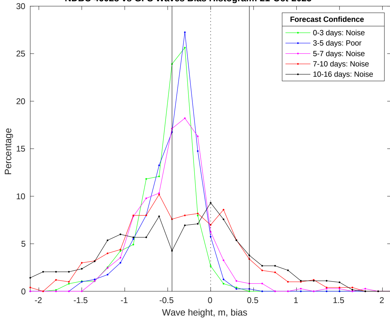
NDBC 46028 vs GFS Waves Bias Histogram: 21-Oct-2025
