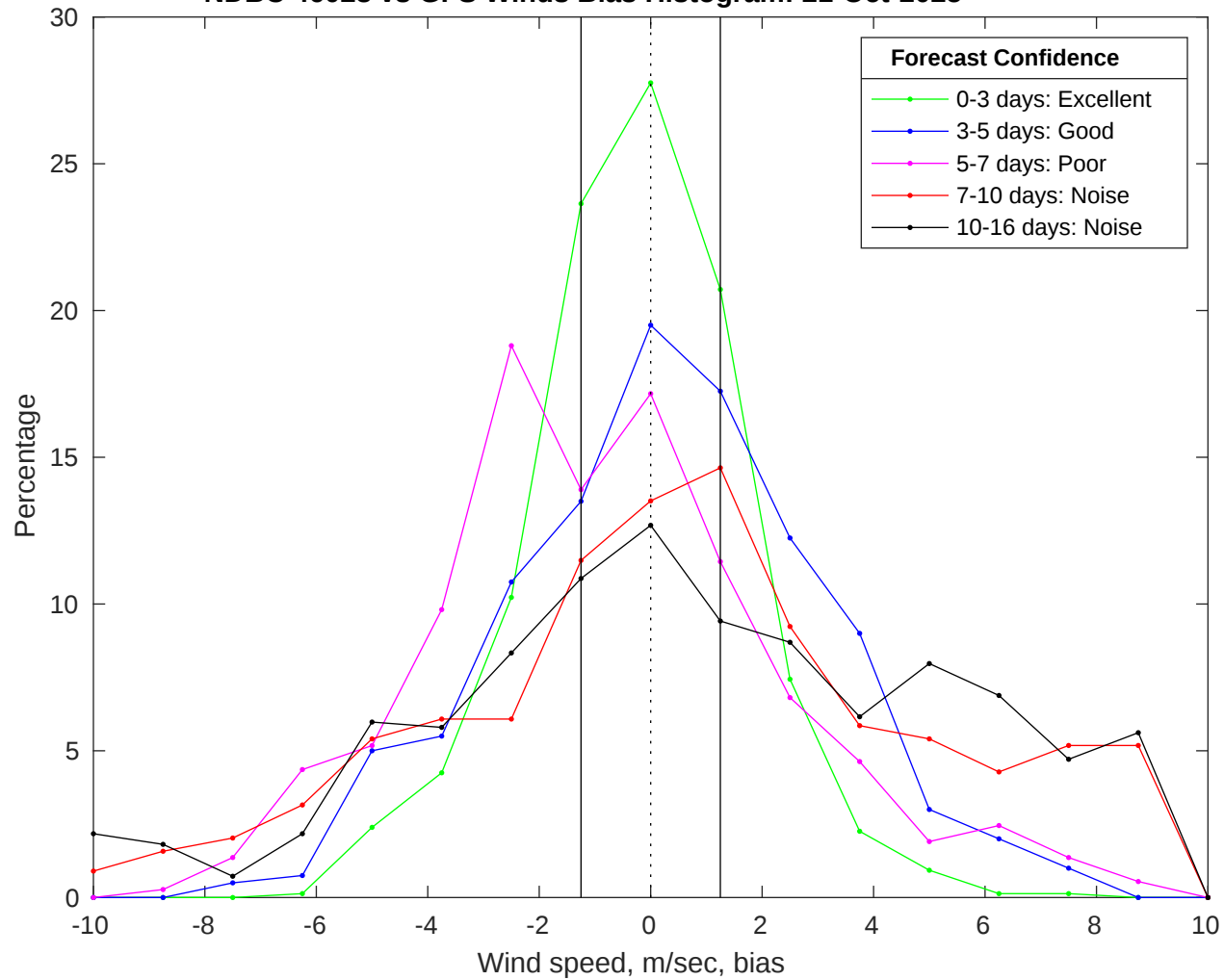
NDBC 46028 vs GFS Winds Bias Histogram: 21-Oct-2025
