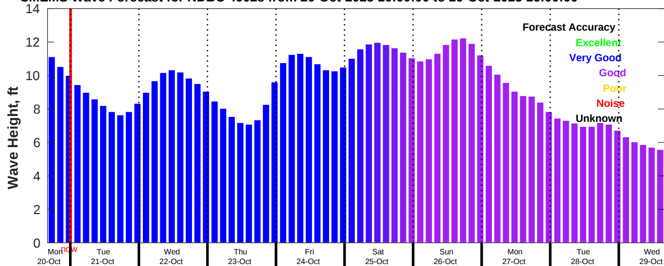
CMEMS Wave Forecast for NDBC 46028 from 20-Oct-2025 16:00:00 to 29-Oct-2025 16:00:00
