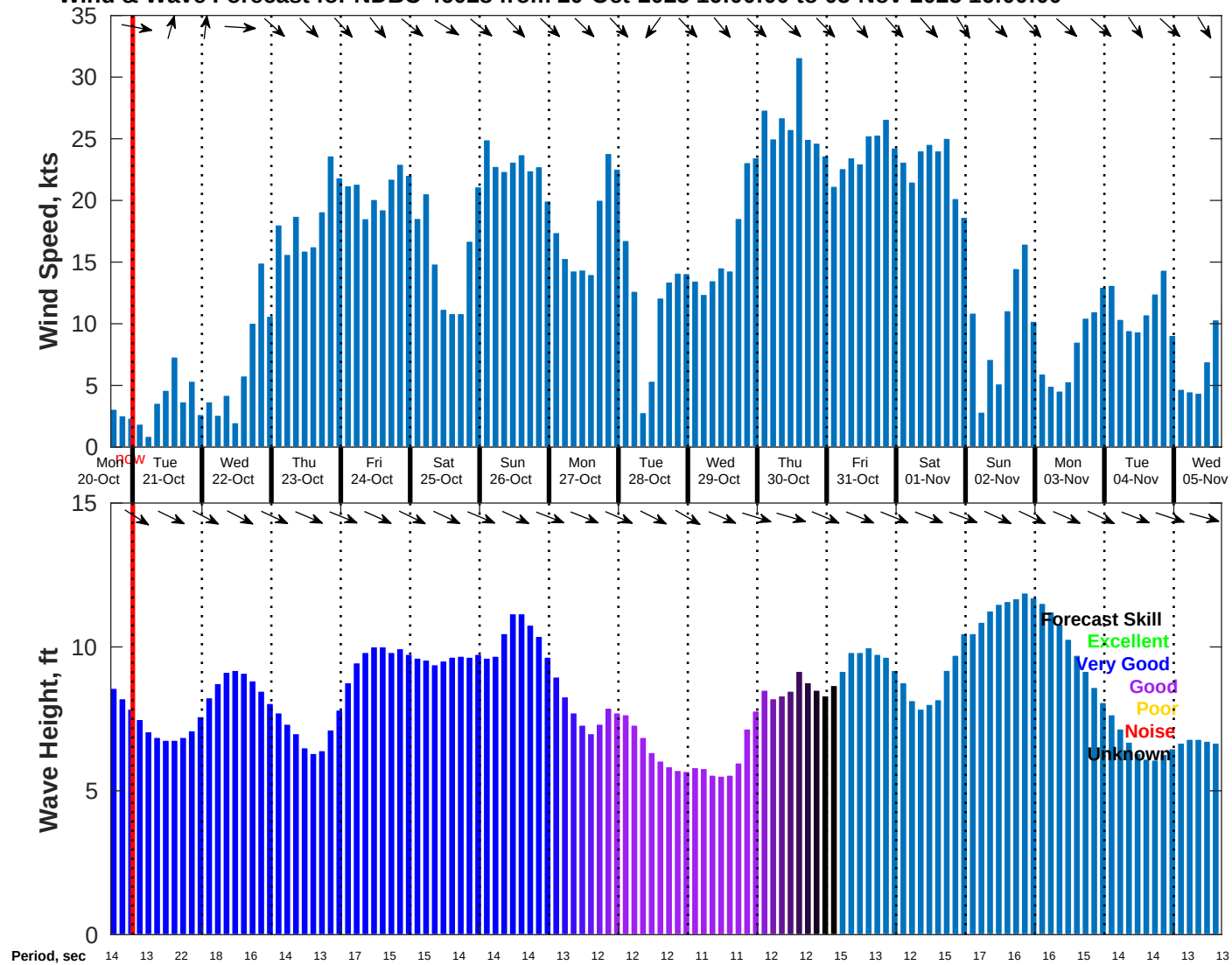
Wind & Wave Forecast for NDBC 46028 from 20-Oct-2025 16:00:00 to 05-Nov-2025 16:00:00
