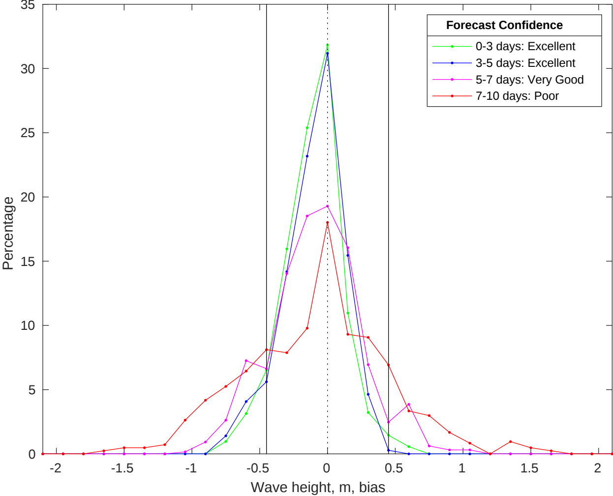
NDBC 46054 vs CMEMS Waves Bias Histogram: 21-Oct-2025
