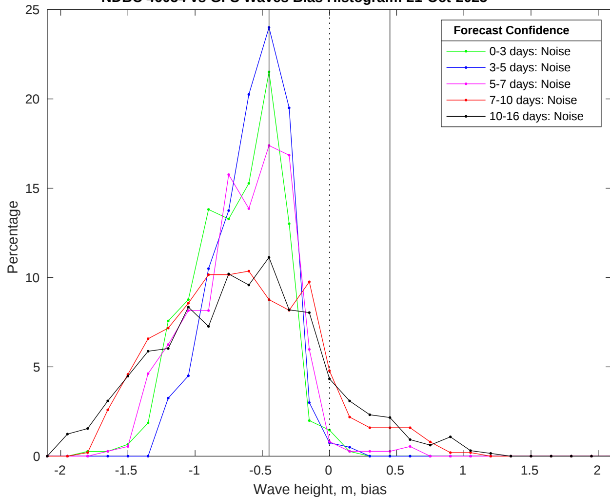
NDBC 46054 vs GFS Waves Bias Histogram: 21-Oct-2025
