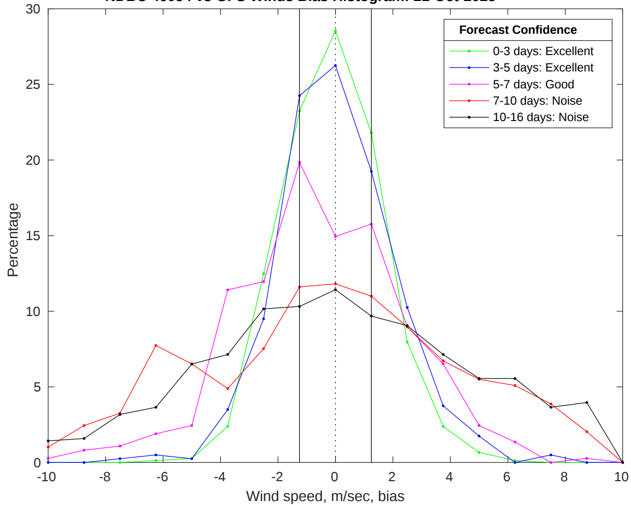
NDBC 46054 vs GFS Winds Bias Histogram: 21-Oct-2025
