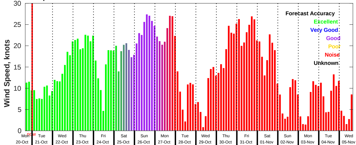
GFS Wind Speed Forecast for NDBC 46054 from 20-Oct-2025 16:00:00 to 05-Nov-2025 16:00:00
