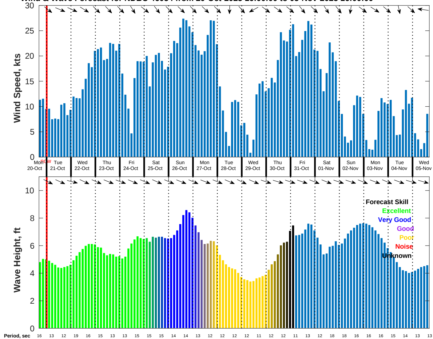
Wind & Wave Forecast for NDBC 46054 from 20-Oct-2025 16:00:00 to 05-Nov-2025 16:00:00
