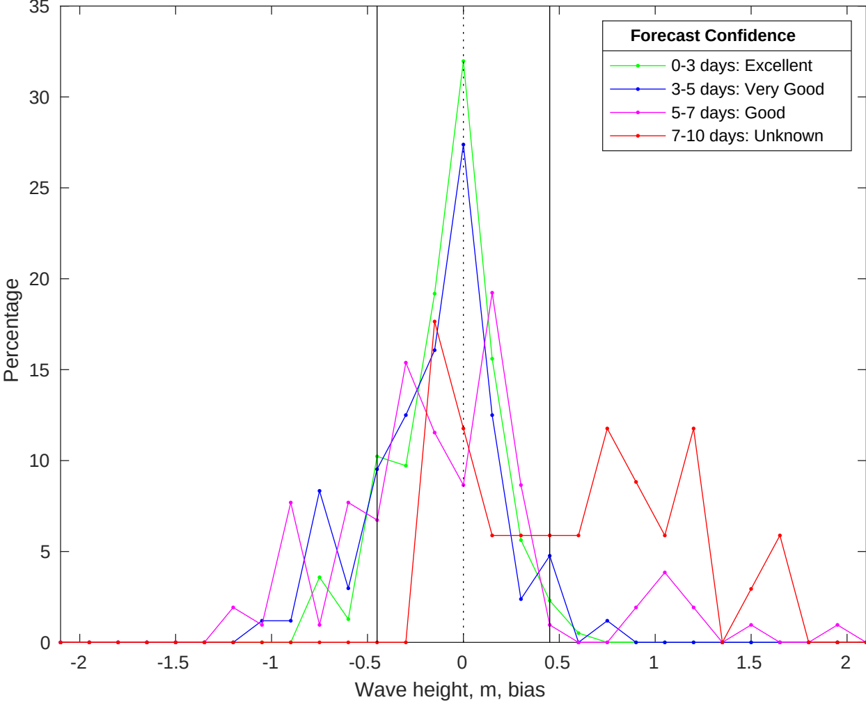
NDBC 46059 vs CMEMS Waves Bias Histogram: 21-Oct-2025
