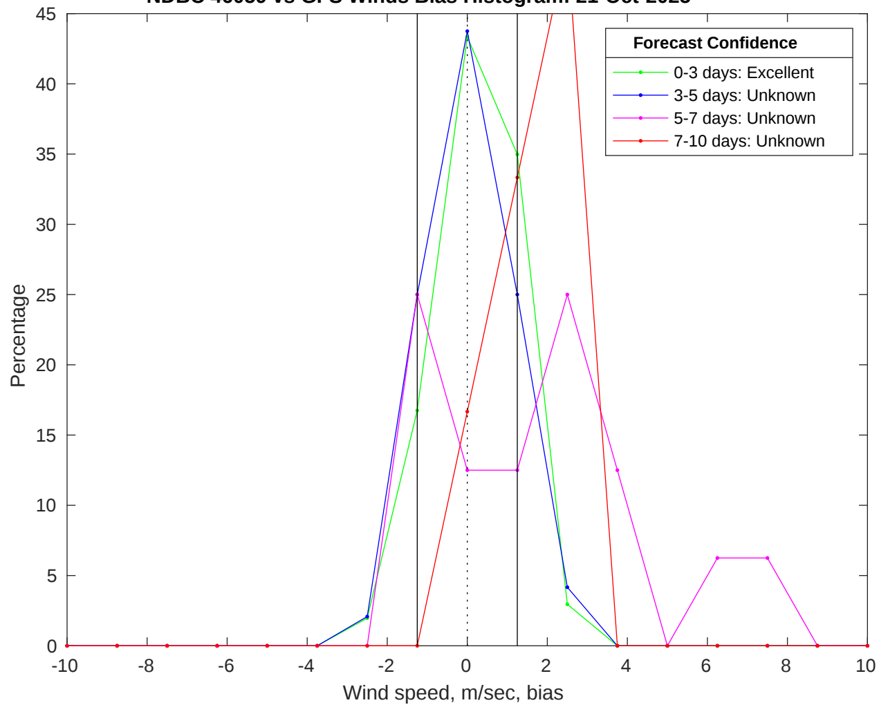
NDBC 46059 vs GFS Winds Bias Histogram: 21-Oct-2025
