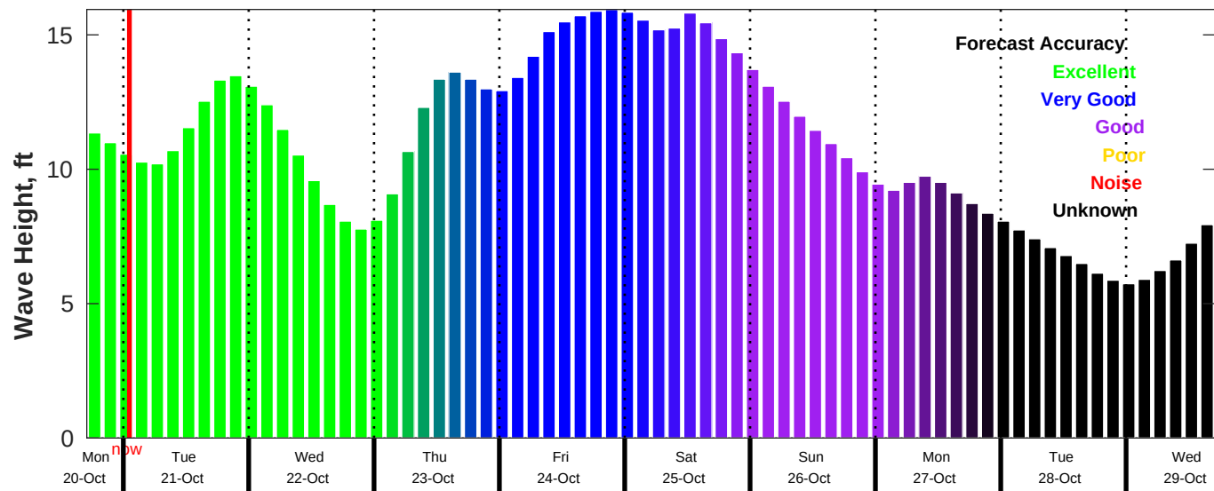
CMEMS Wave Forecast for NDBC 46059 from 20-Oct-2025 17:00:00 to 29-Oct-2025 17:00:00
